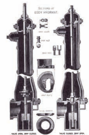
FIG. 140.—Eddy Fire Hydrant.
